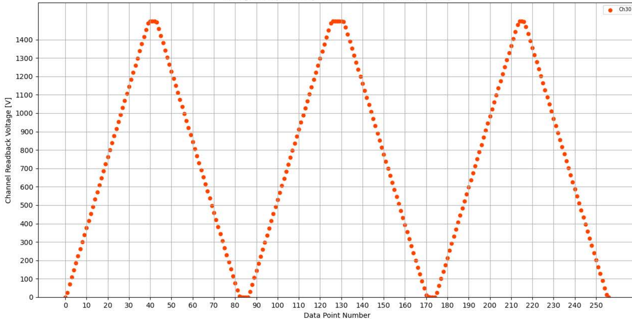
Voltage Ramp Test (Python) Bd #324, Slot #7, Ch #30
