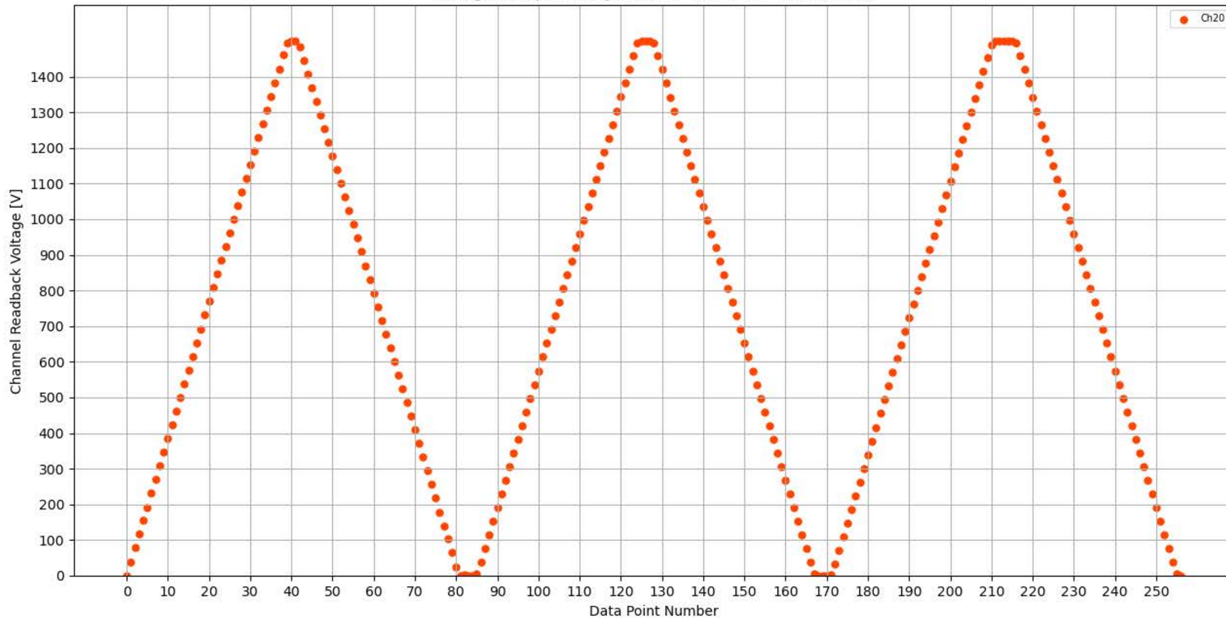
Voltage Ramp Test (Python) Bd #324, Slot #7, Ch #20
