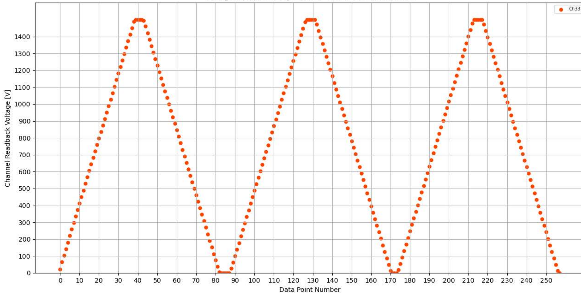
Voltage Ramp Test (Python) Bd #324, Slot #7, Ch #33
