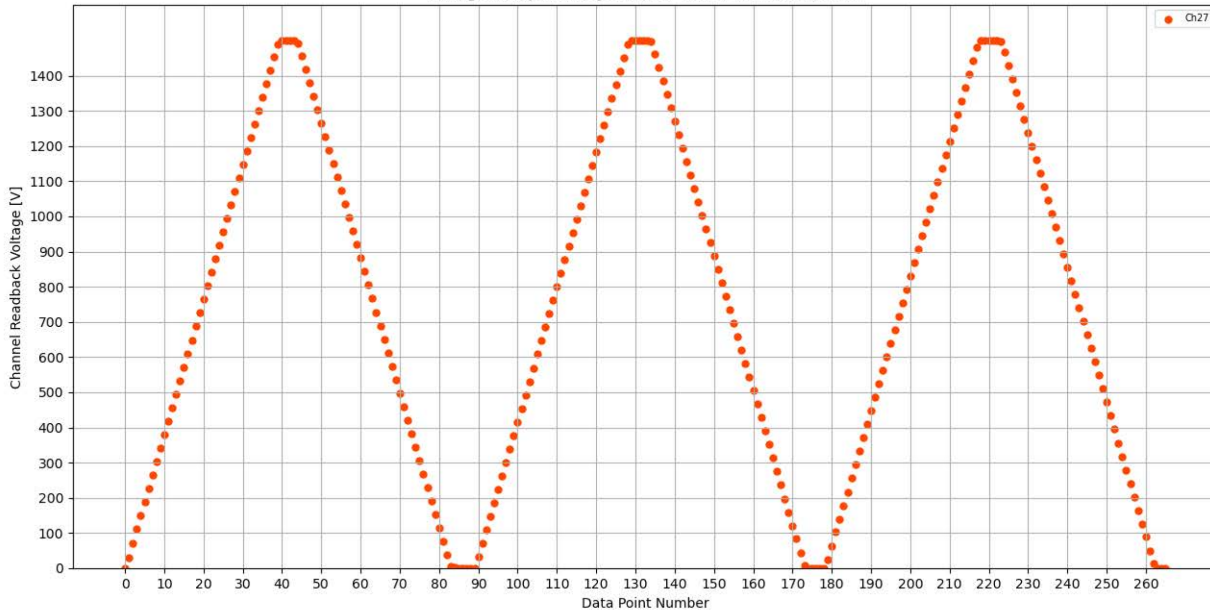
Voltage Ramp Test (Python) Bd #324, Slot #7, Ch #27
