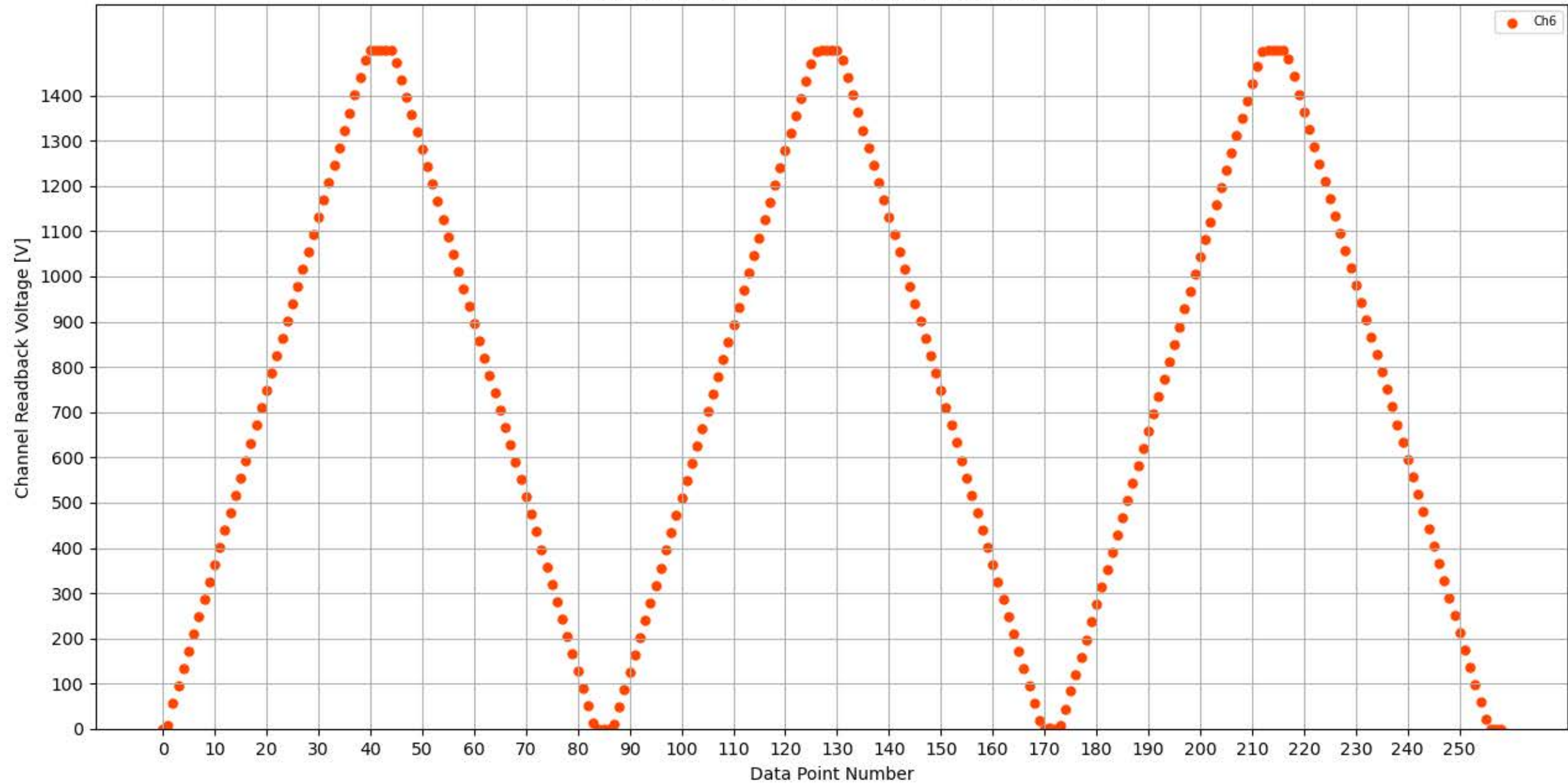
Voltage Ramp Test (Python) Bd #324, Slot #7, Ch #6
