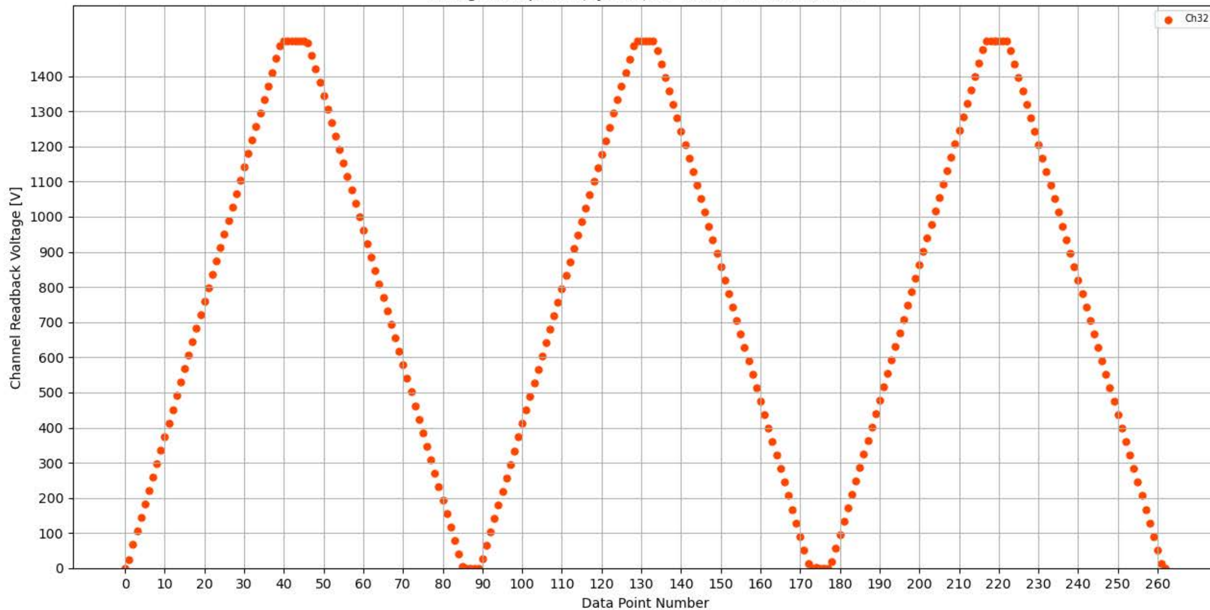
Voltage Ramp Test (Python) Bd #324, Slot #7, Ch #32
