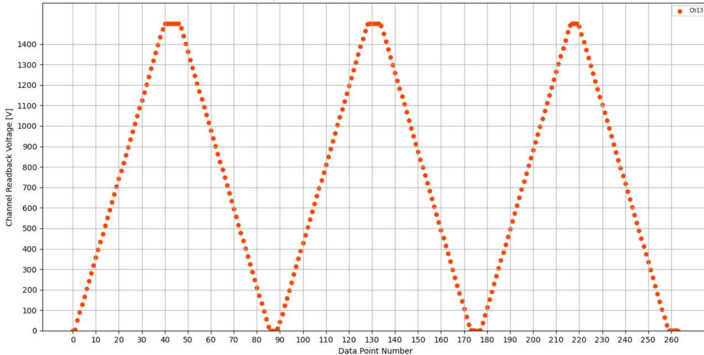
Voltage Ramp Test (Python) Bd #324, Slot #7, Ch #13
