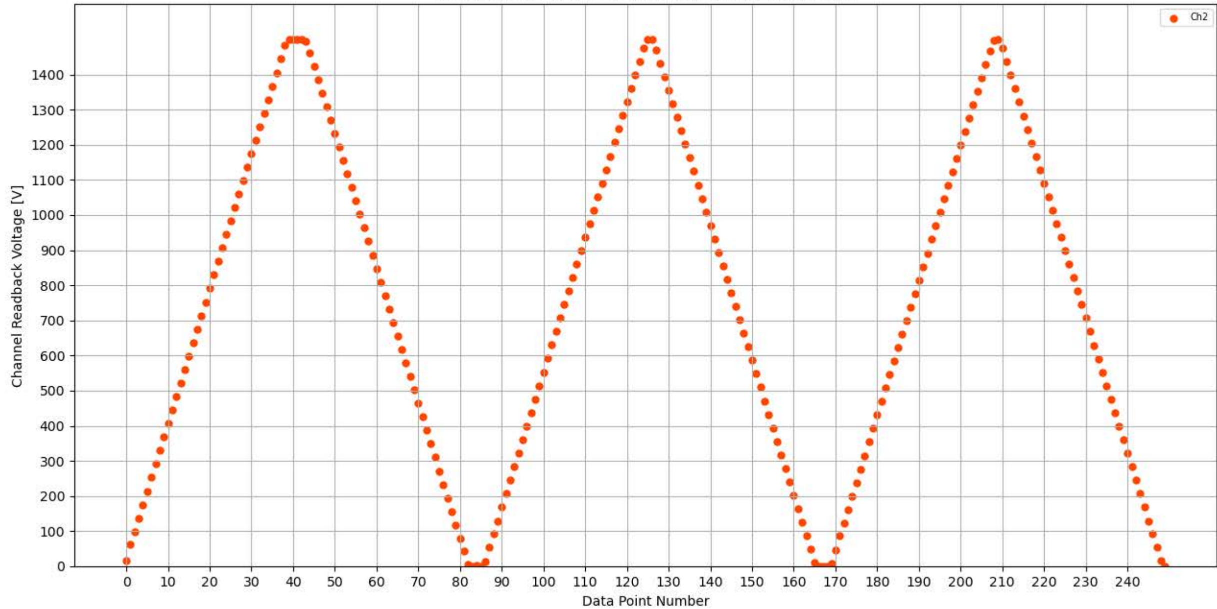
Voltage Ramp Test (Python) Bd #324, Slot #7, Ch #2
