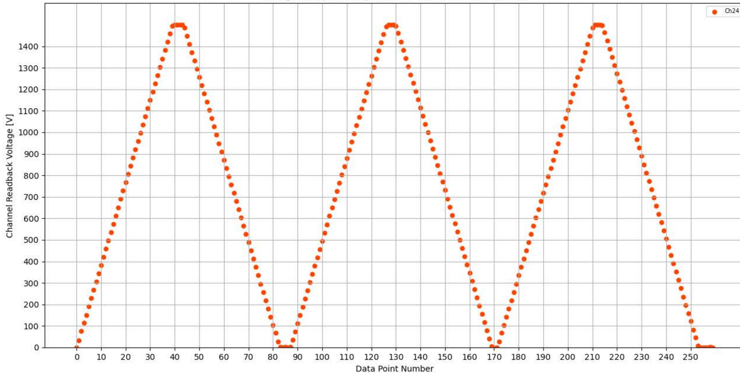
Voltage Ramp Test (Python) Bd #324, Slot #7, Ch #24
