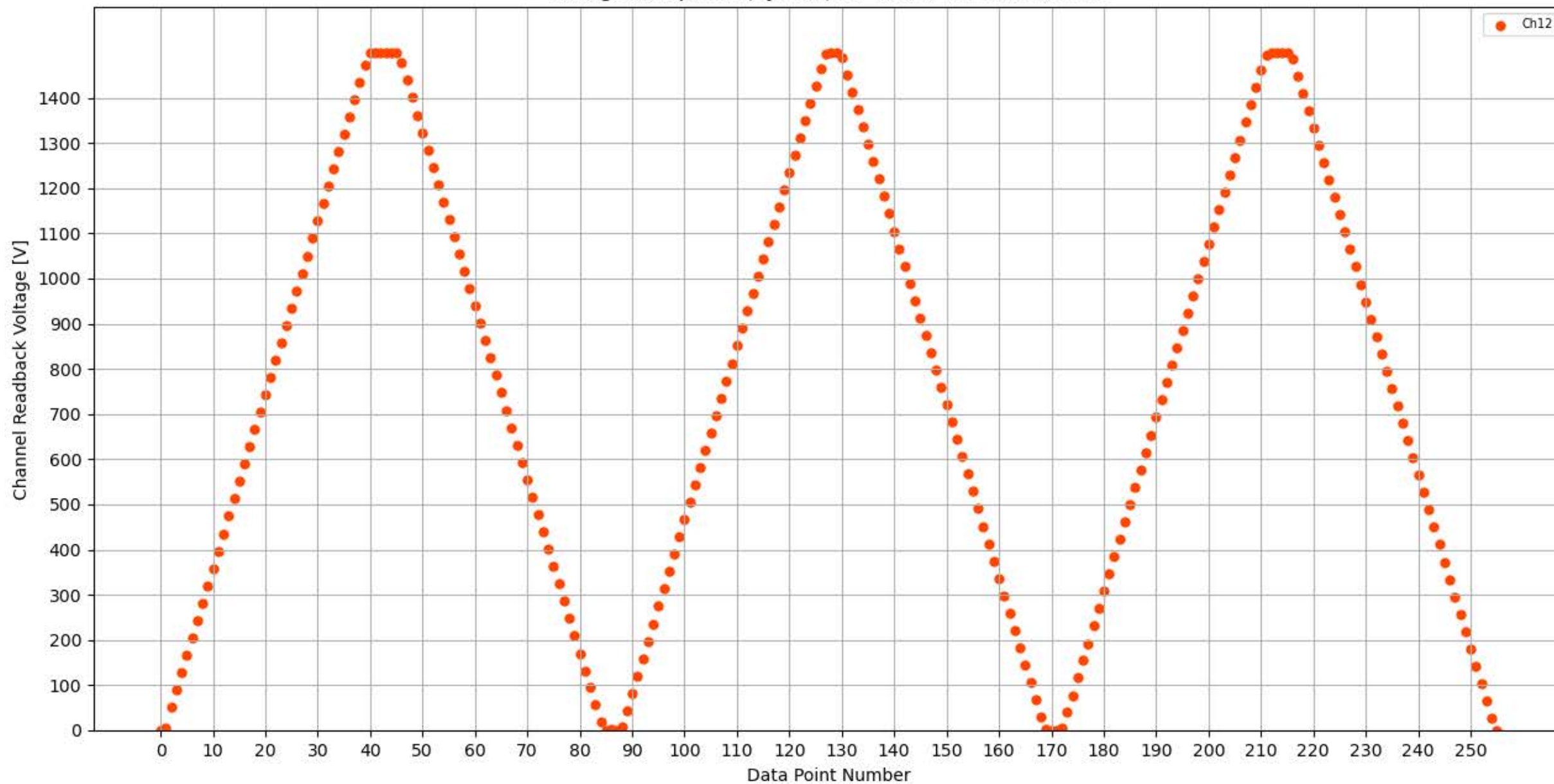
Voltage Ramp Test (Python) Bd #324, Slot #7, Ch #12
