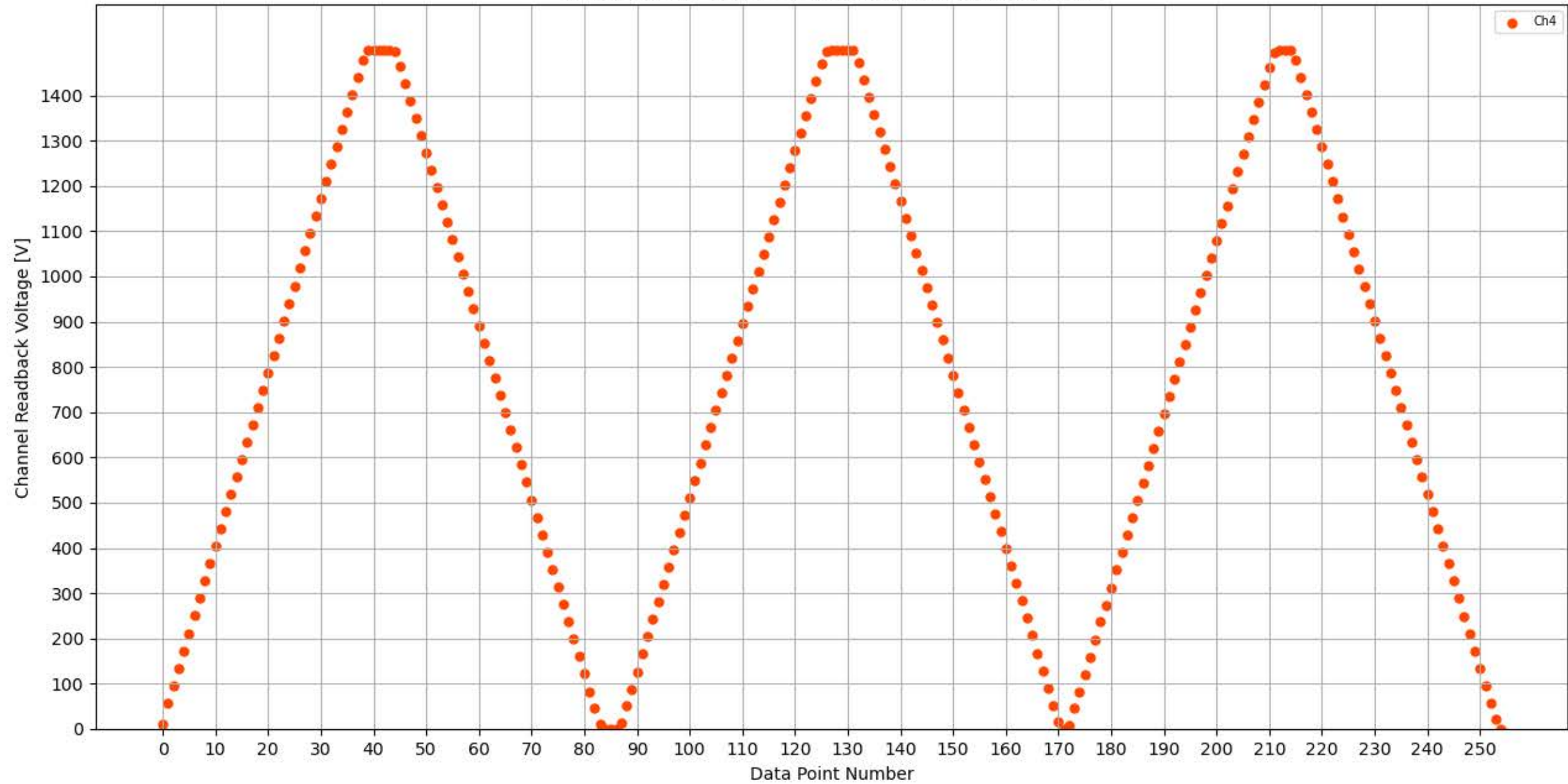
Voltage Ramp Test (Python) Bd #324, Slot #7, Ch #4
