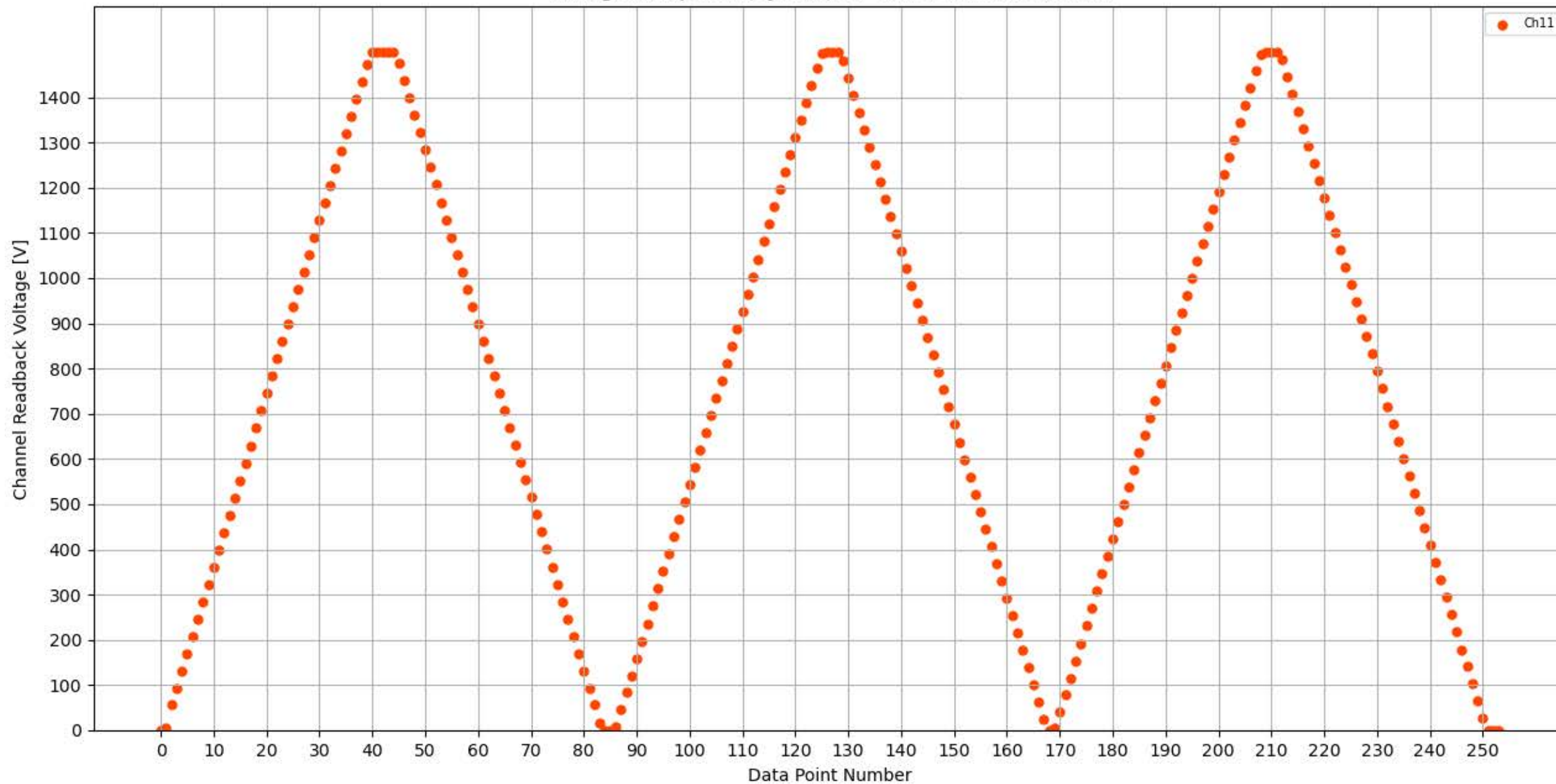
Voltage Ramp Test (Python) Bd #324, Slot #7, Ch #11
