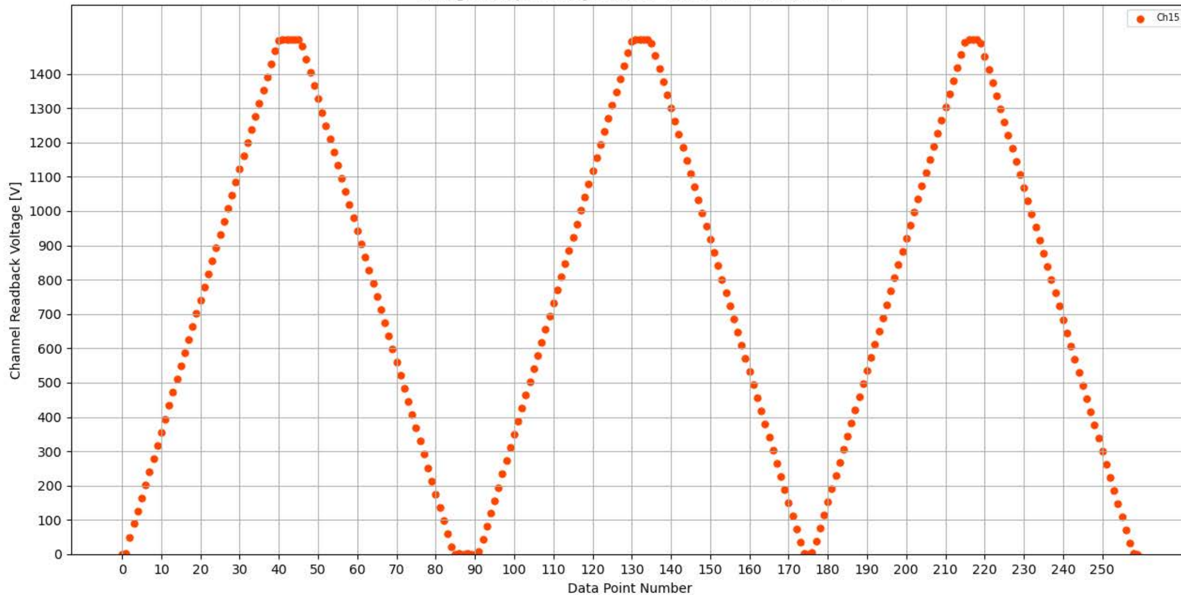
Voltage Ramp Test (Python) Bd #324, Slot #7, Ch #15
