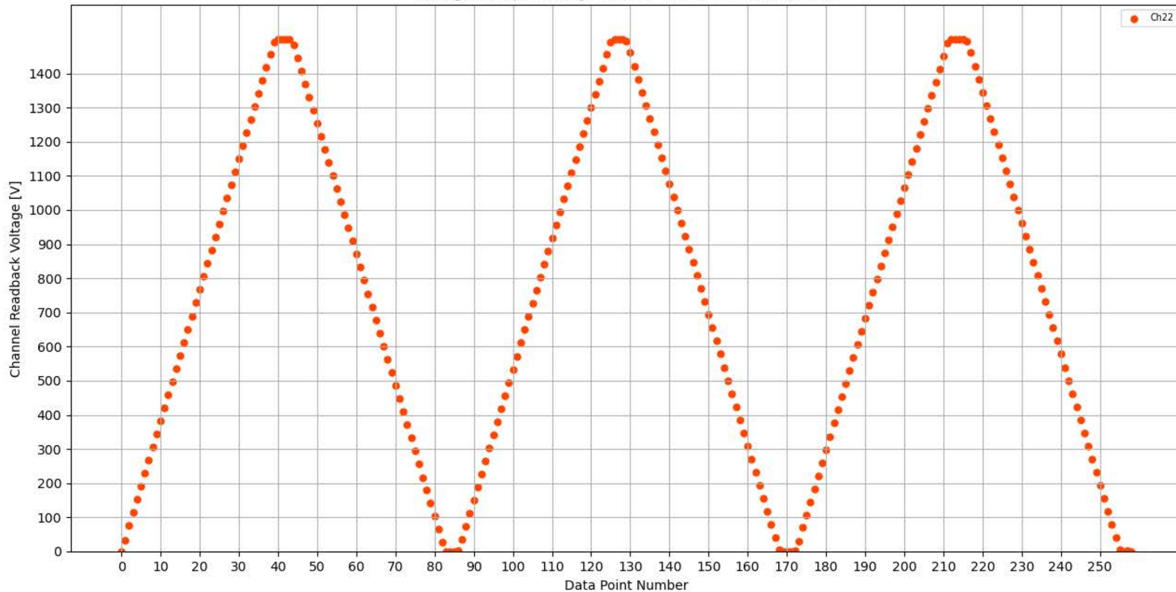
Voltage Ramp Test (Python) Bd #324, Slot #7, Ch #22
