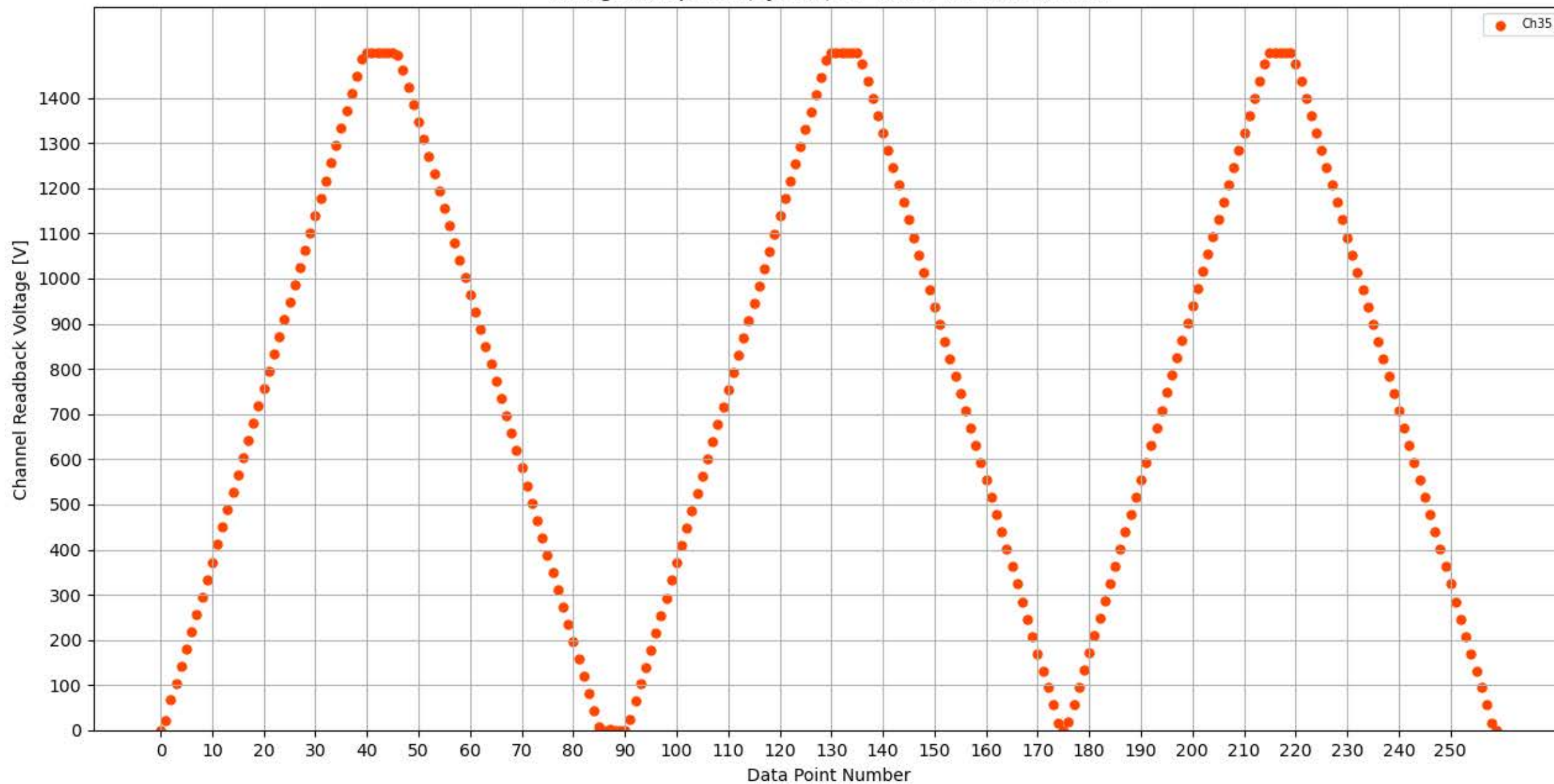
Voltage Ramp Test (Python) Bd #324, Slot #7, Ch #35
