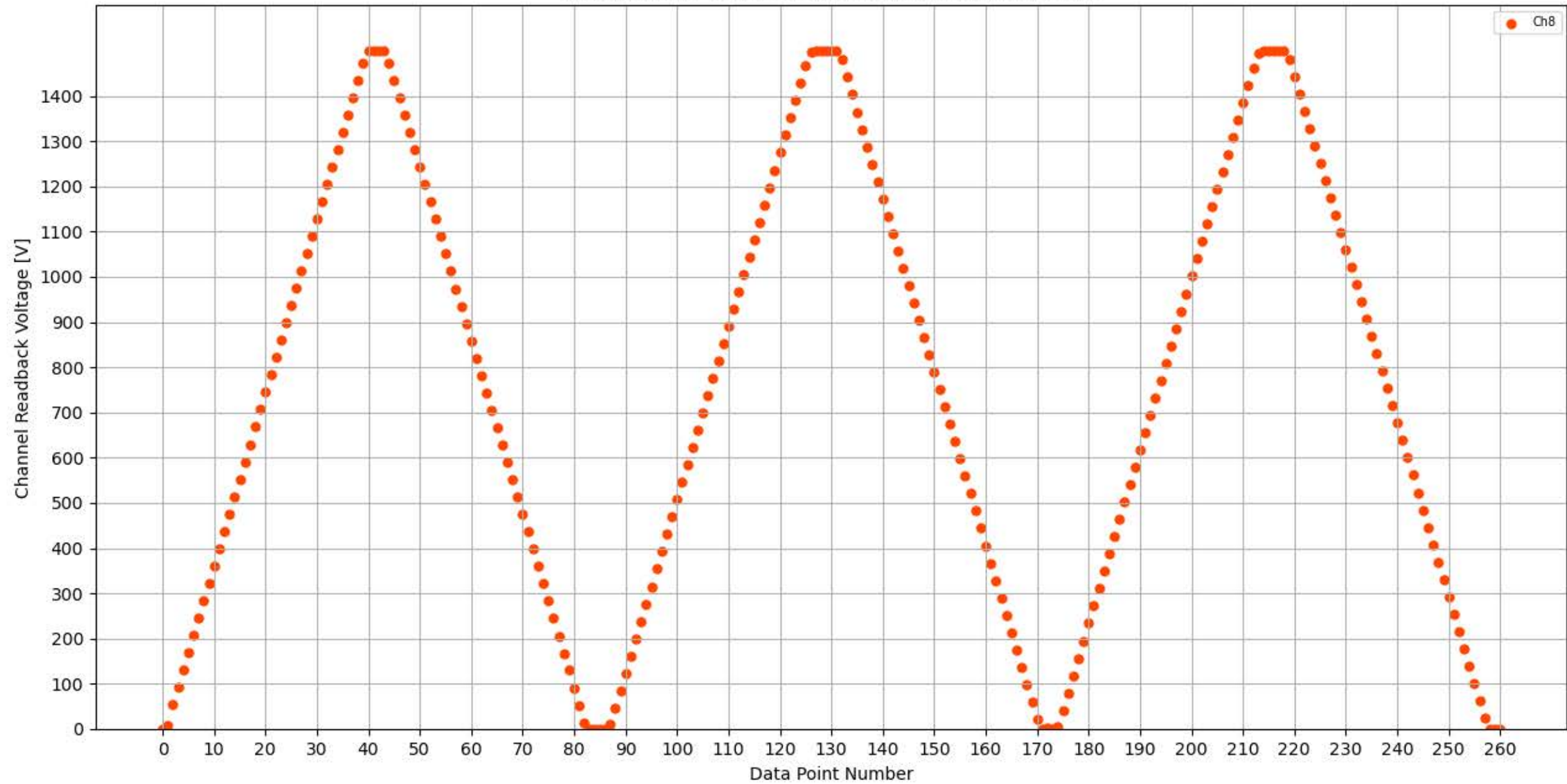
Voltage Ramp Test (Python) Bd #324, Slot #7, Ch #8
