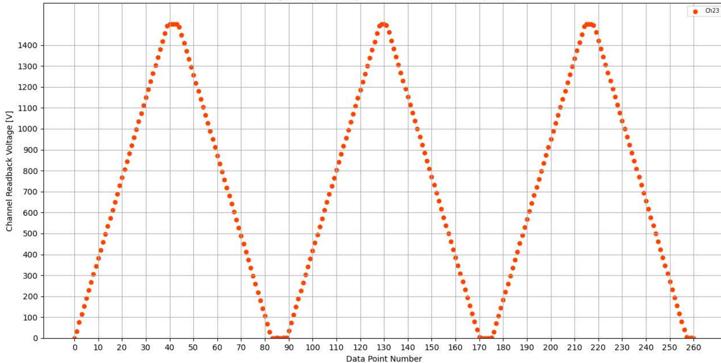
Voltage Ramp Test (Python) Bd #324, Slot #7, Ch #23
