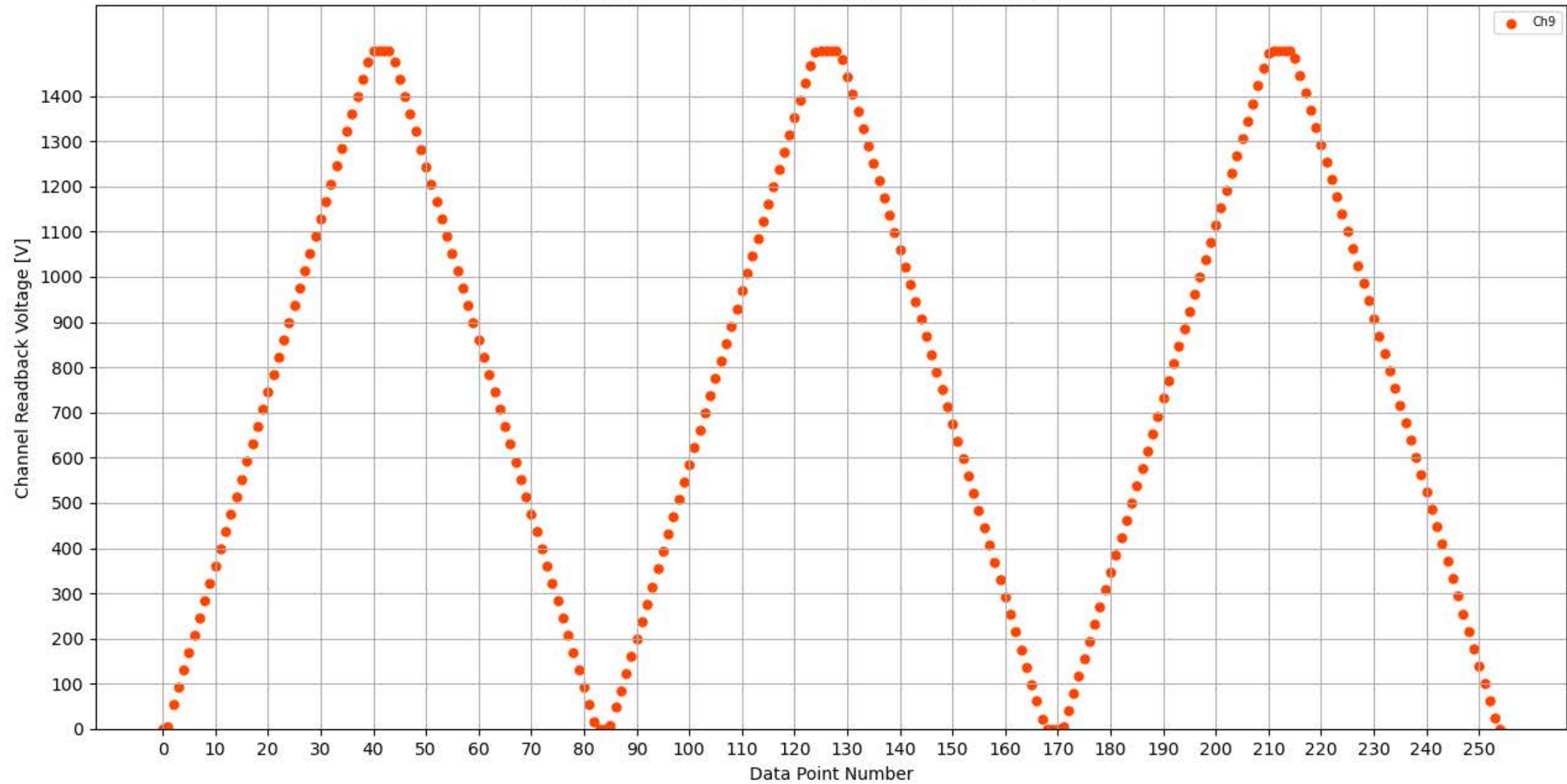
Voltage Ramp Test (Python) Bd #324, Slot #7, Ch #9
