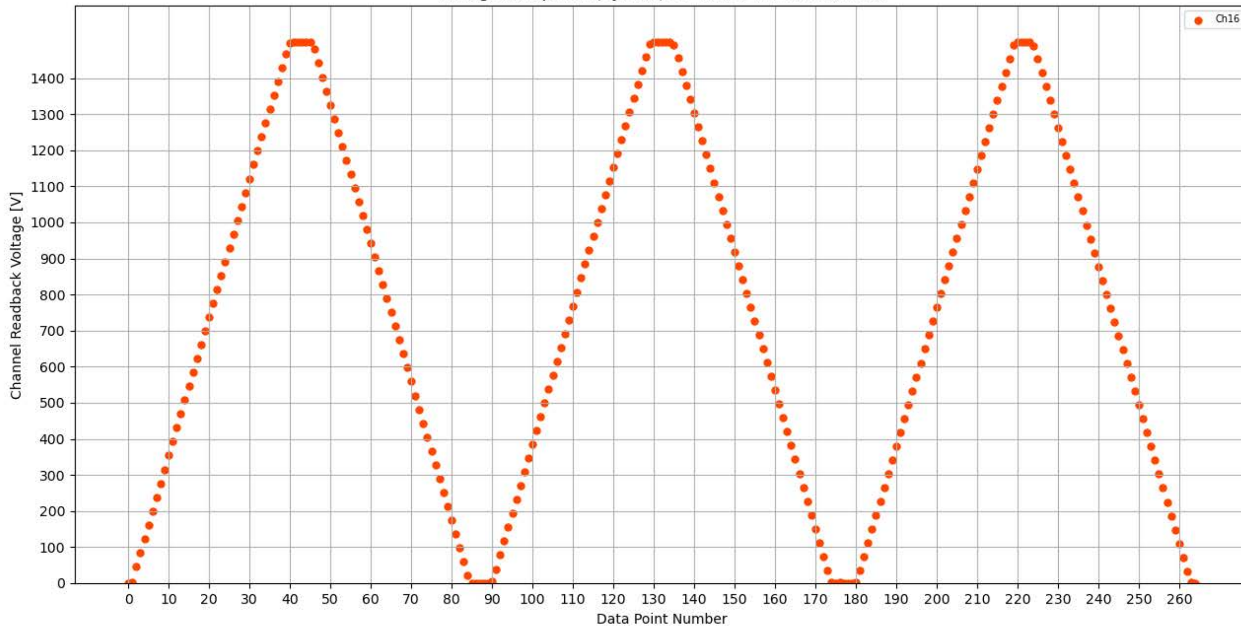
Voltage Ramp Test (Python) Bd #324, Slot #7, Ch #16
