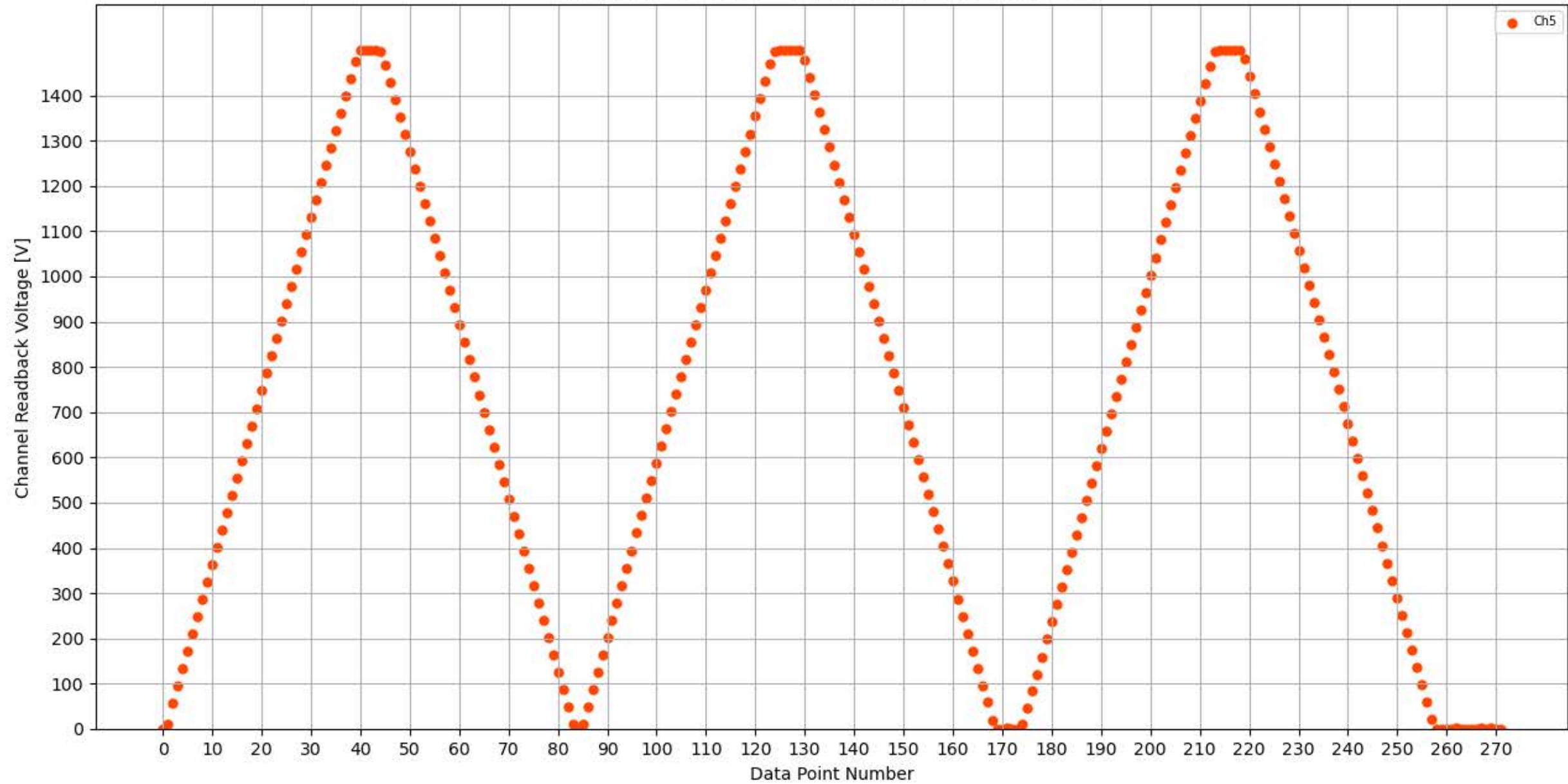
Voltage Ramp Test (Python) Bd #324, Slot #7, Ch #5
