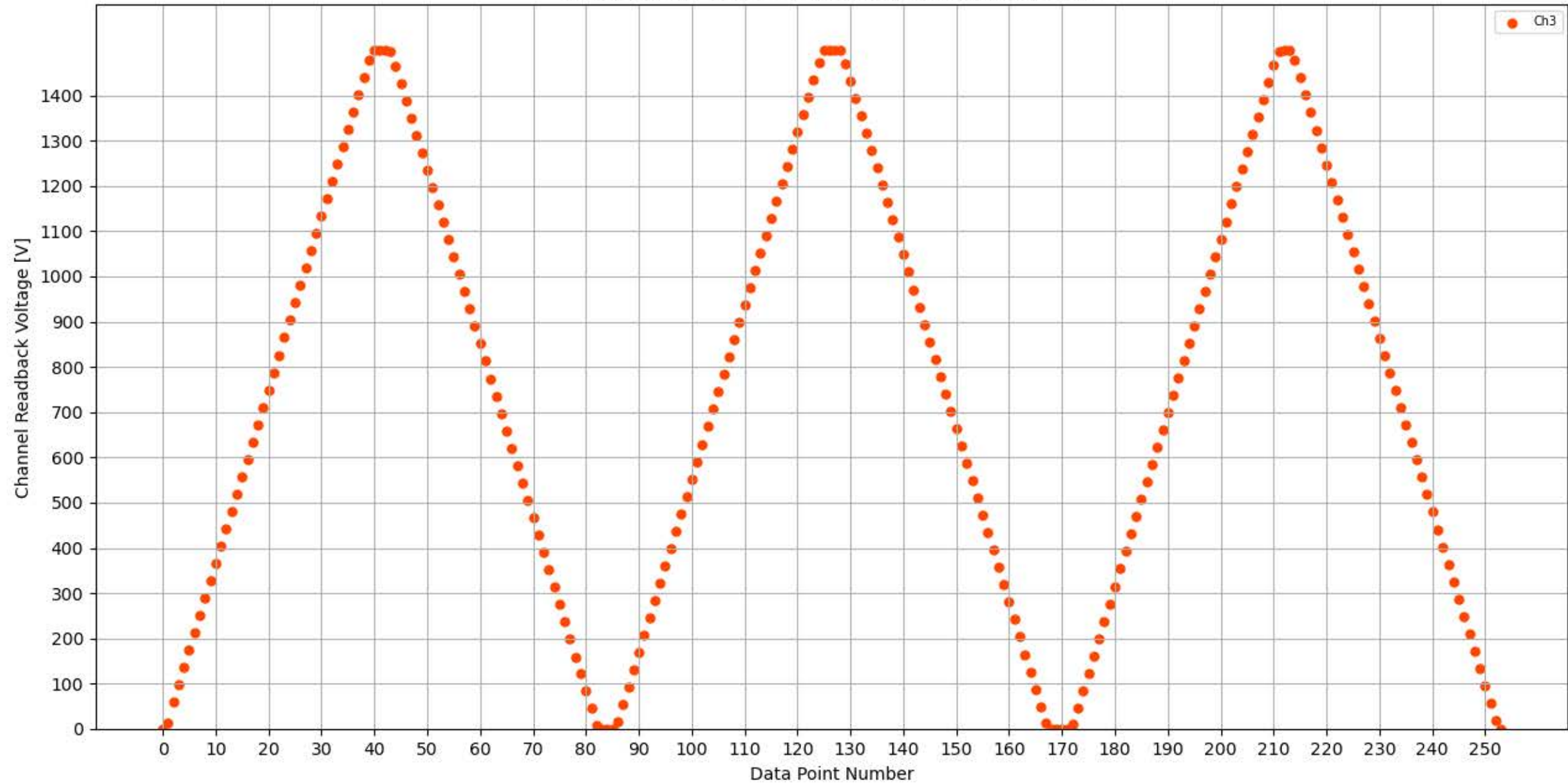
Voltage Ramp Test (Python) Bd #324, Slot #7, Ch #3
