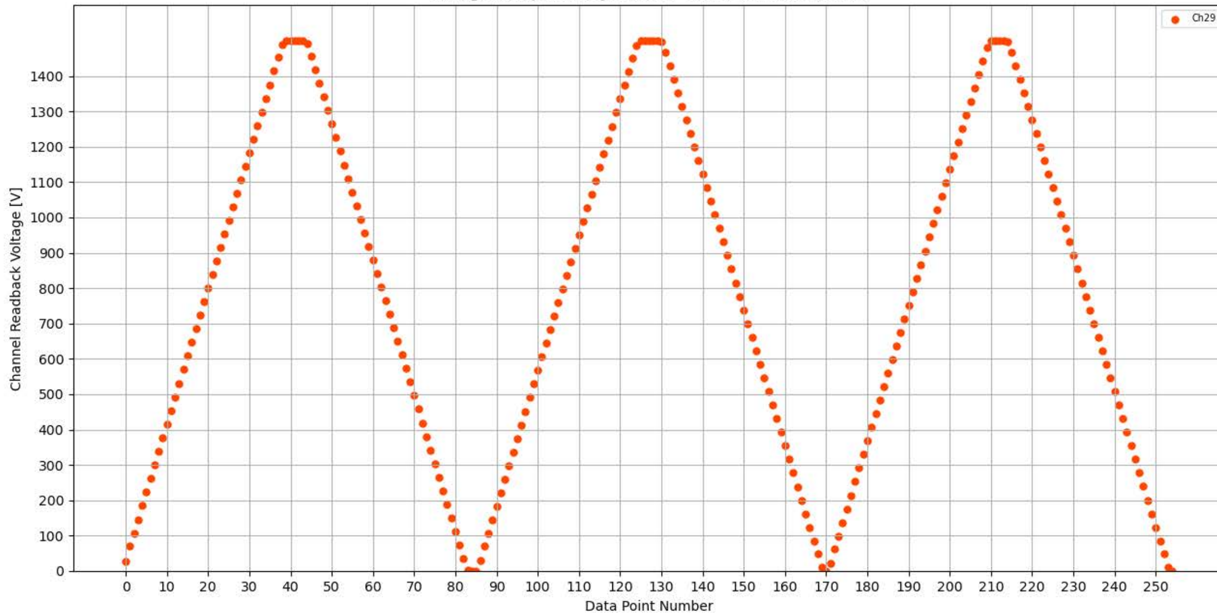
Voltage Ramp Test (Python) Bd #324, Slot #7, Ch #29
