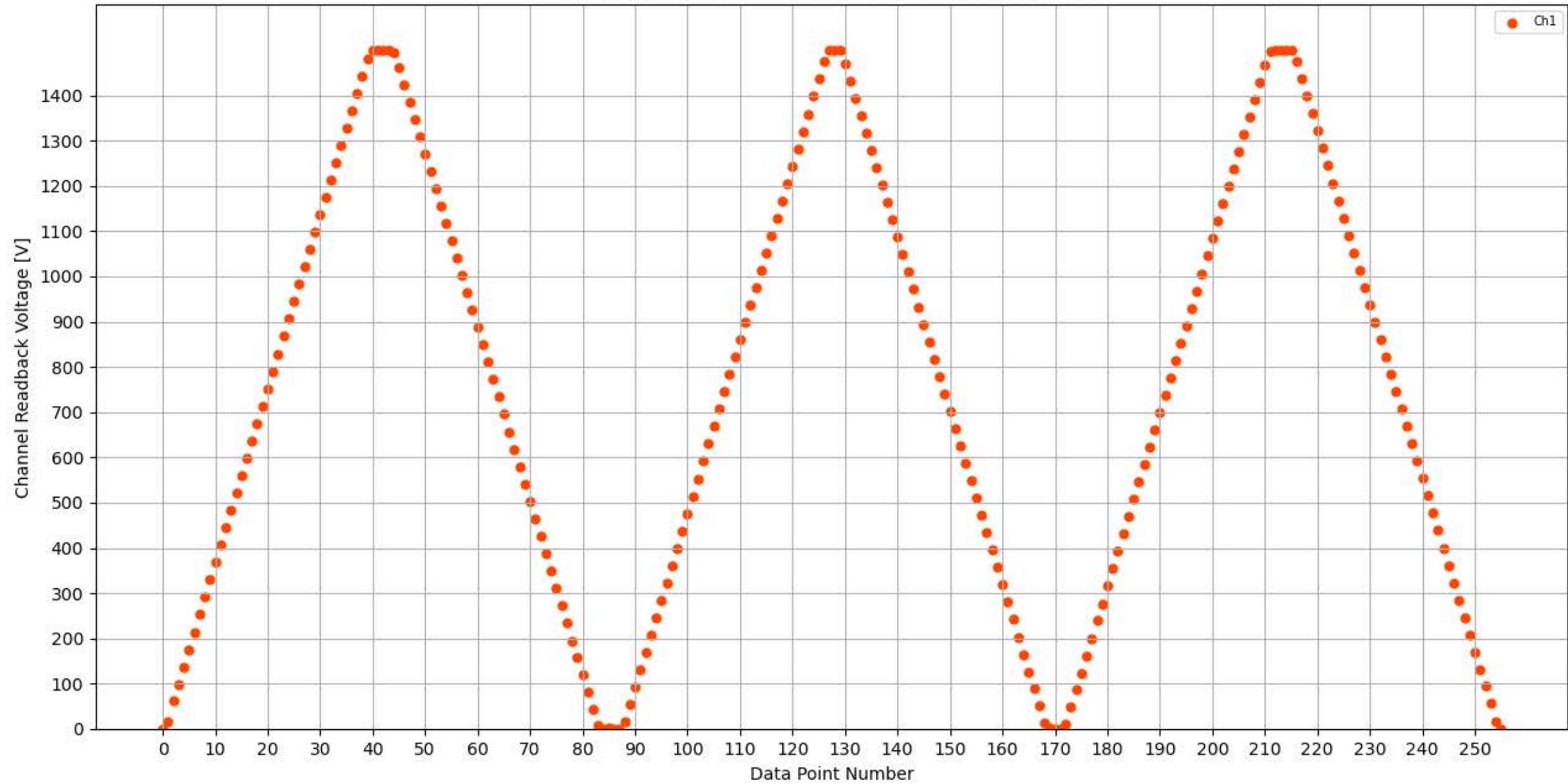
Voltage Ramp Test (Python) Bd #324, Slot #7, Ch #1
