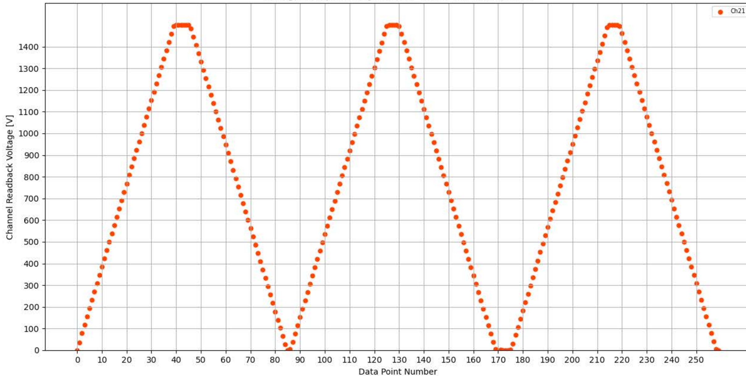
Voltage Ramp Test (Python) Bd #324, Slot #7, Ch #21
