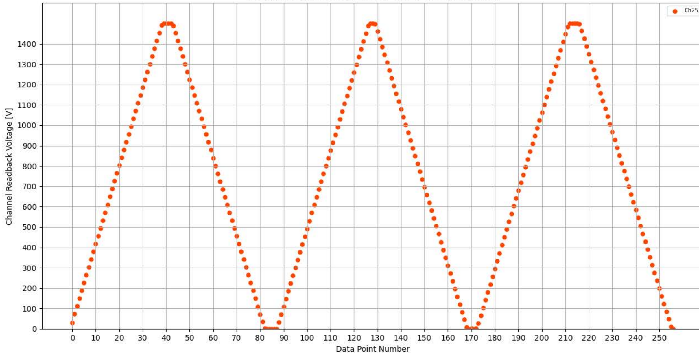
Voltage Ramp Test (Python) Bd #324, Slot #7, Ch #25
