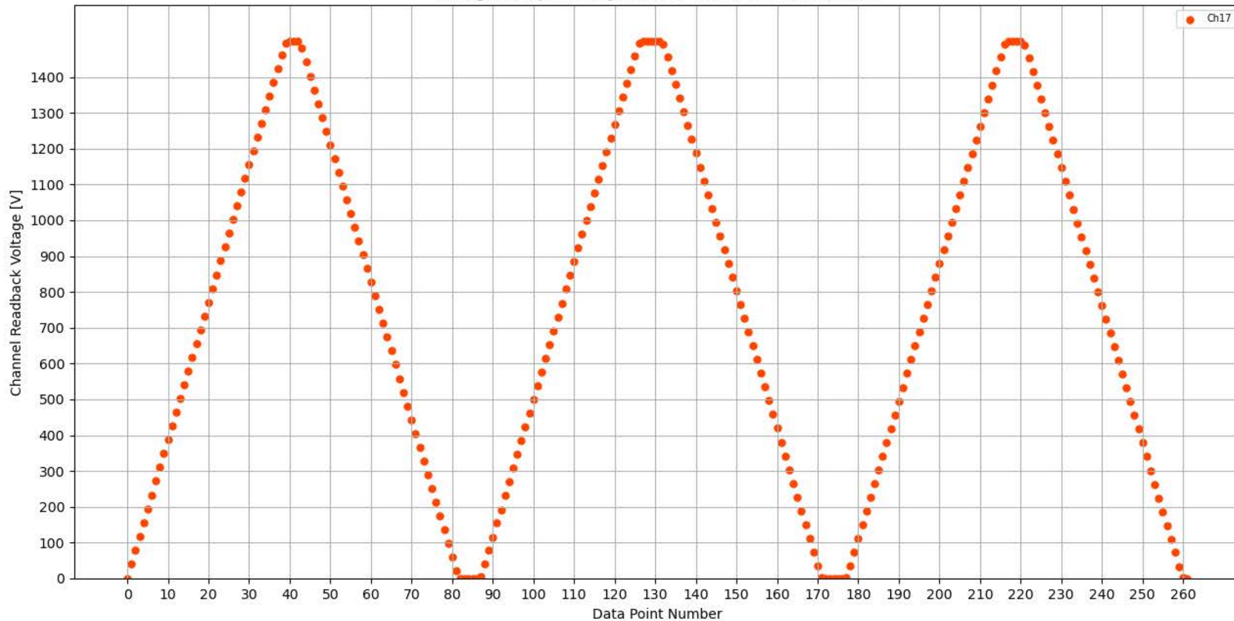
Voltage Ramp Test (Python) Bd #324, Slot #7, Ch #17
