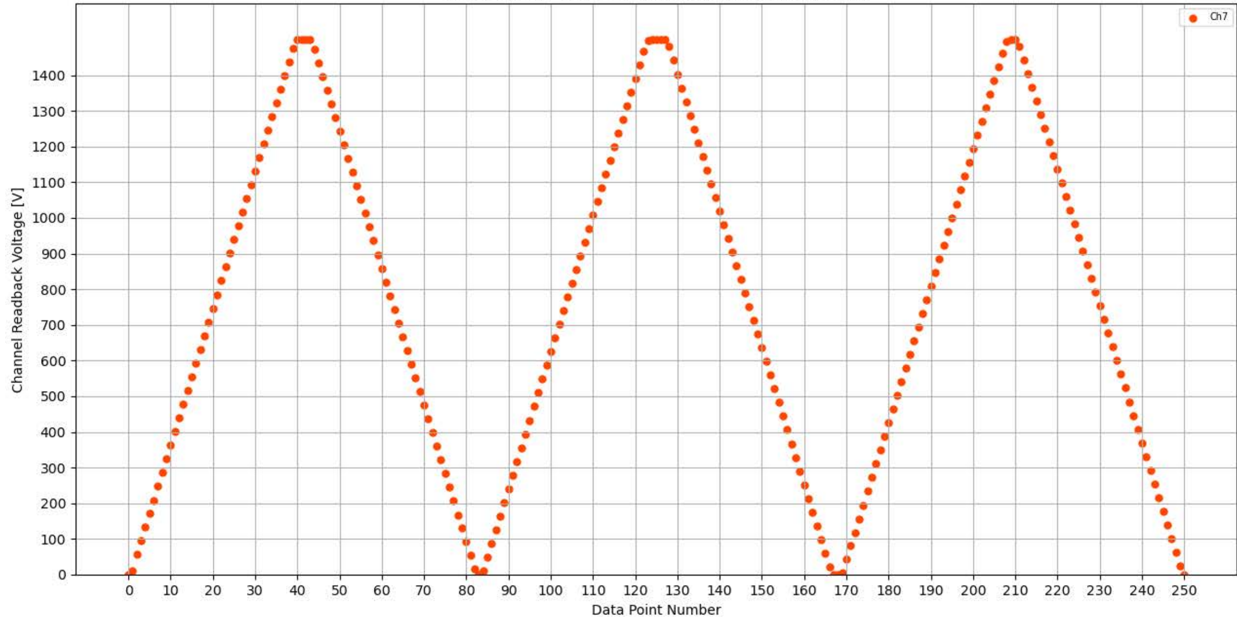
Voltage Ramp Test (Python) Bd #324, Slot #7, Ch #7
