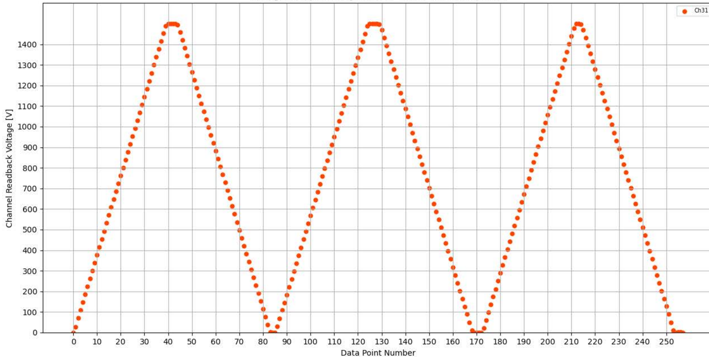
Voltage Ramp Test (Python) Bd #324, Slot #7, Ch #31
