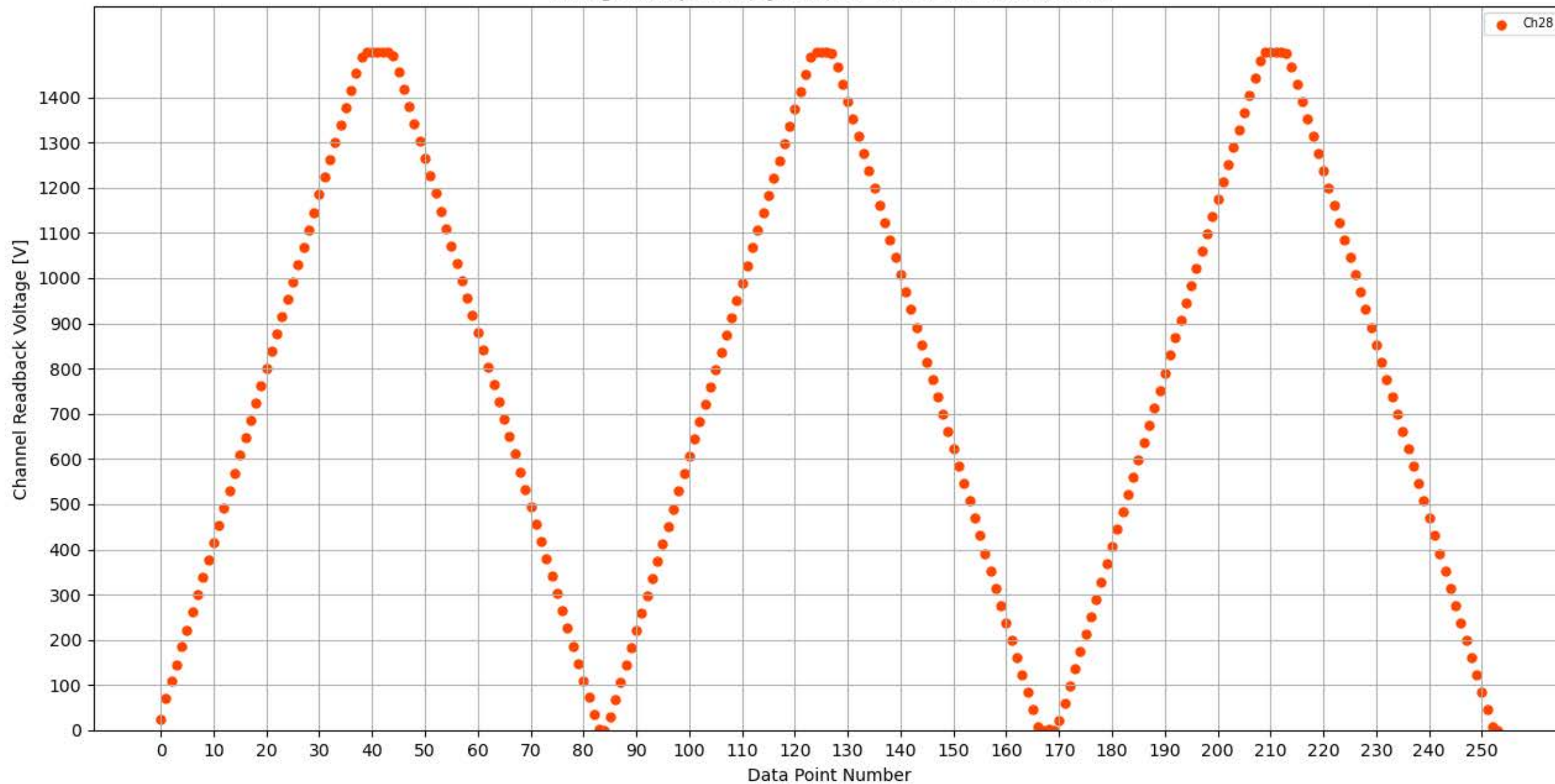
Voltage Ramp Test (Python) Bd #324, Slot #7, Ch #28
