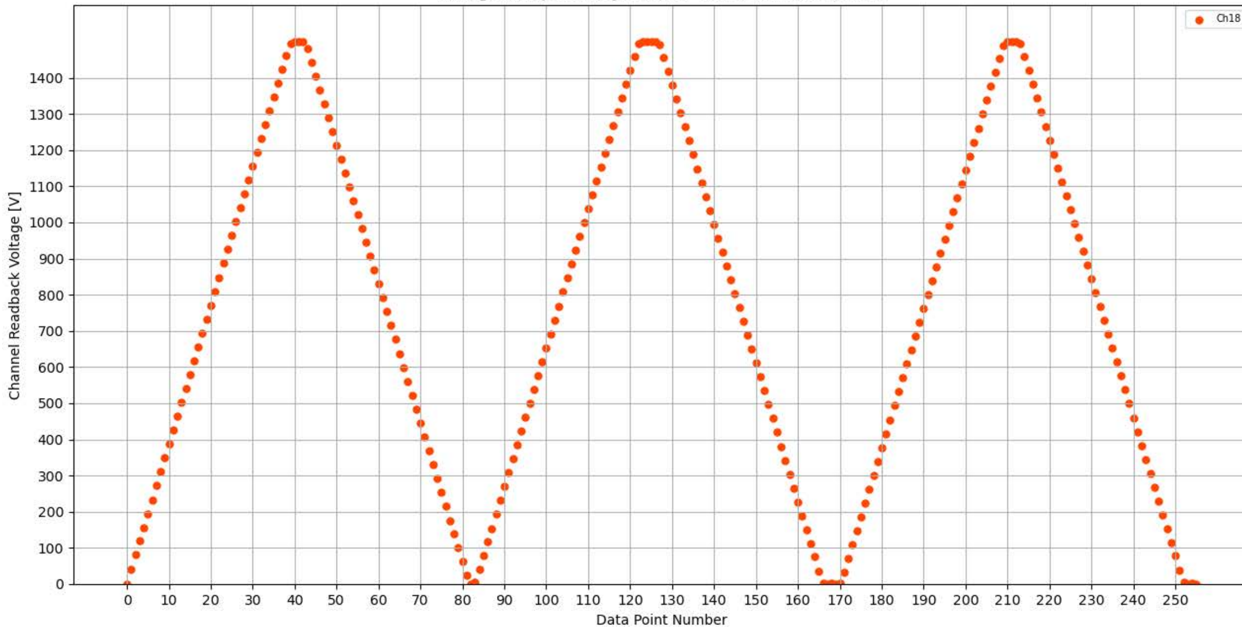
Voltage Ramp Test (Python) Bd #324, Slot #7, Ch #18
