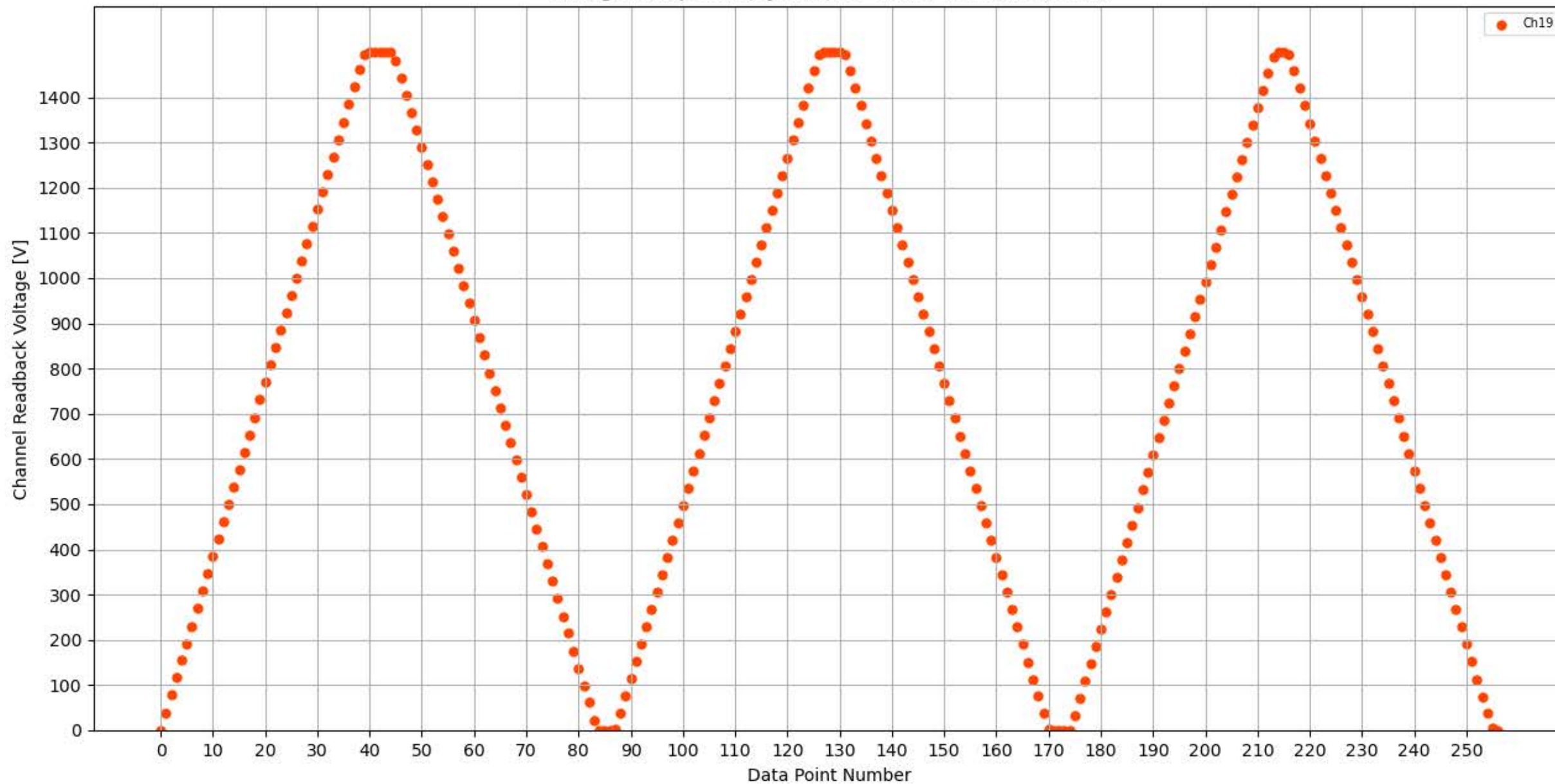
Voltage Ramp Test (Python) Bd #324, Slot #7, Ch #19
